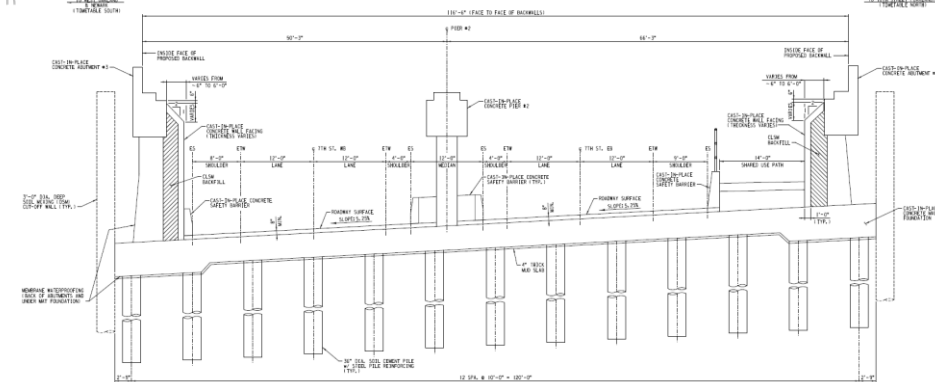
Cross section 2
