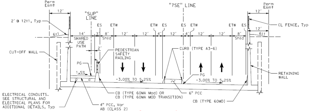
Cross section 1
